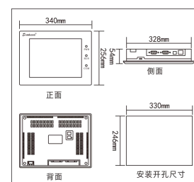
SK-121FS
