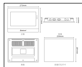
SK-102QS/QT
