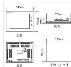
SK-121FE
